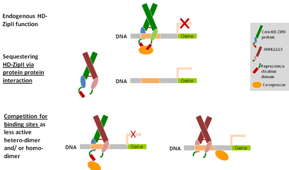
Figure 8: Proposed mechanism of action of the ATHB17 \Delta 113 protein (diagram taken from Figure S2 of Rice et al (2014))
